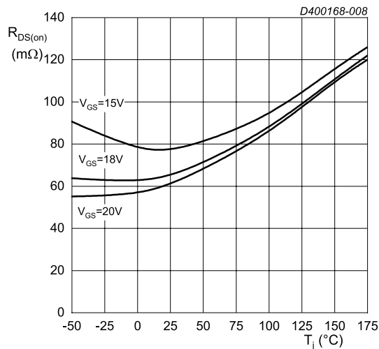
I_{DS} = 20\text{ A}; t_p < 200\text{ }\mu\text{s} Fig. 8. Drain-source on-state resistance as a function of junction temperature
